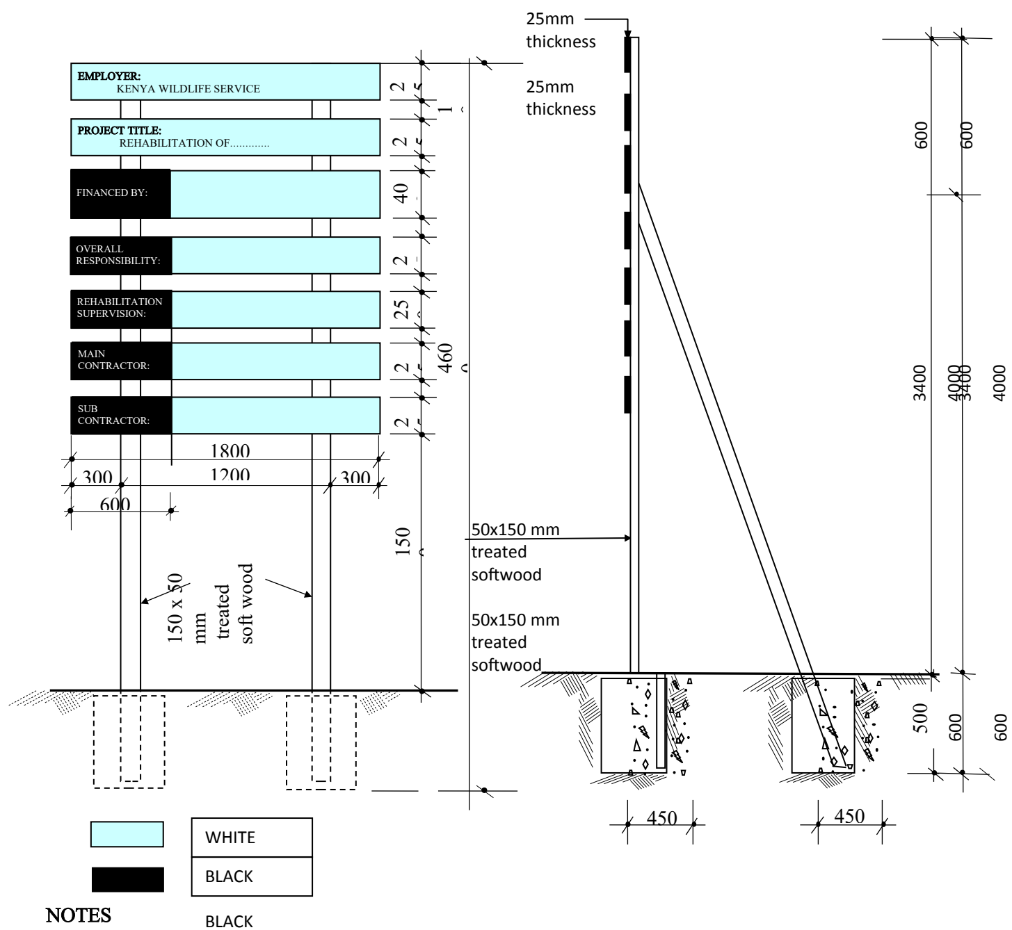
FIGURE C.17 - PUBLICITY SIGNBOARD
