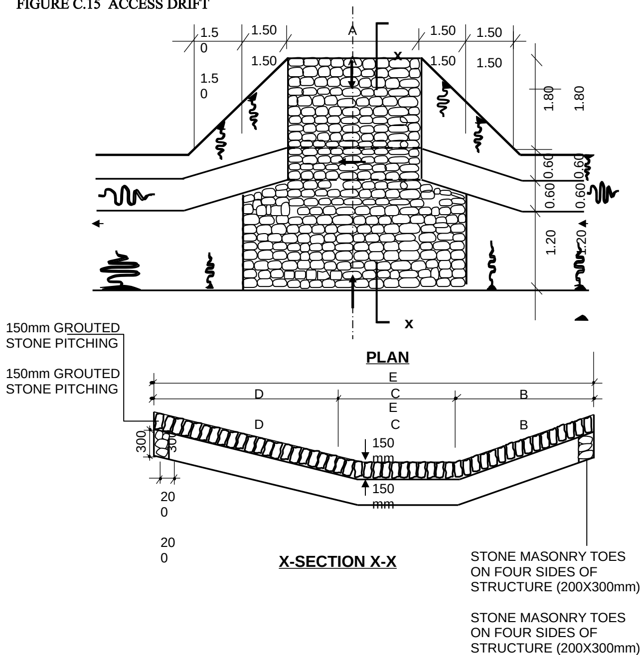
FIGURE C.15 ACCESS DRIFT
