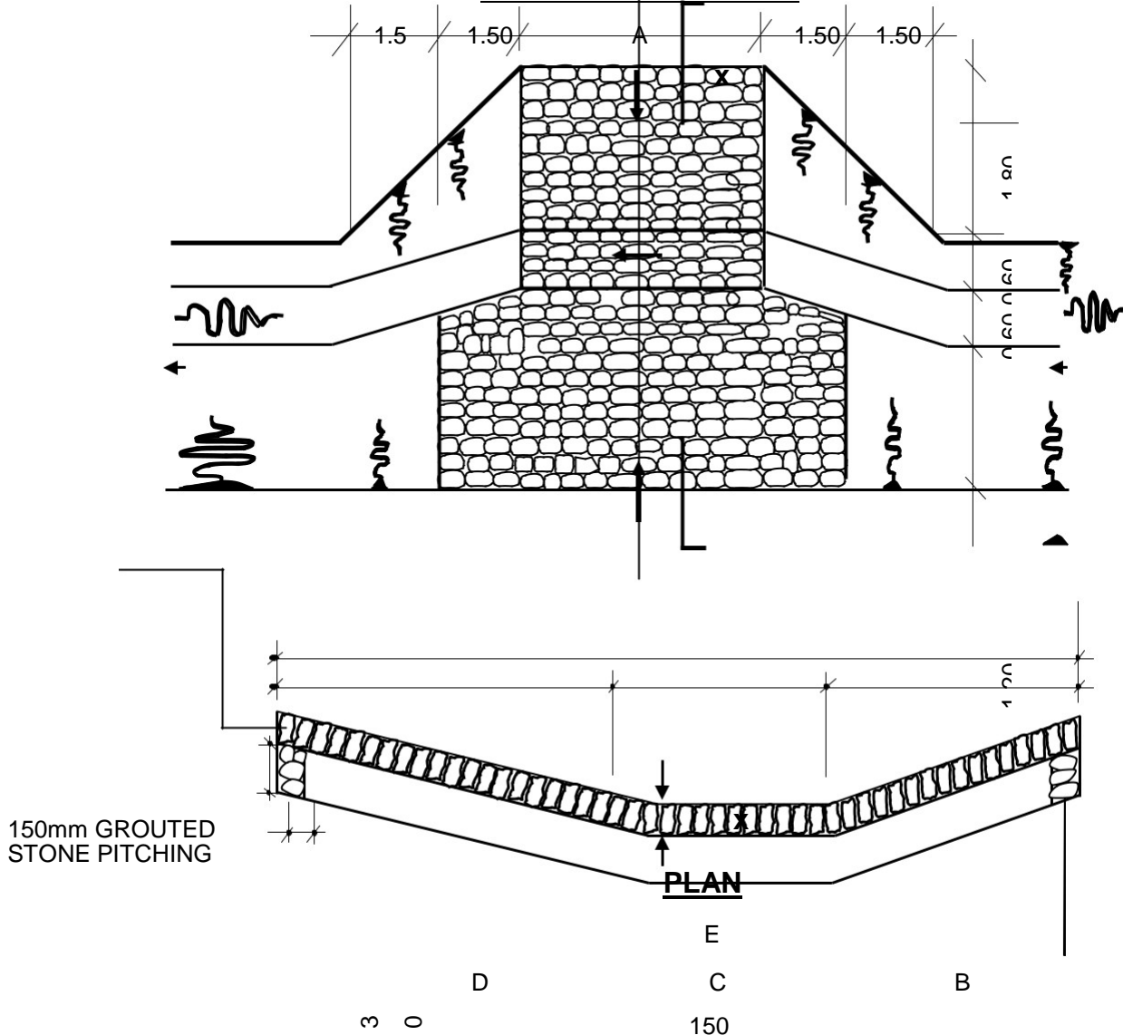
FIGURE C.15 ACCESS DRIFT
