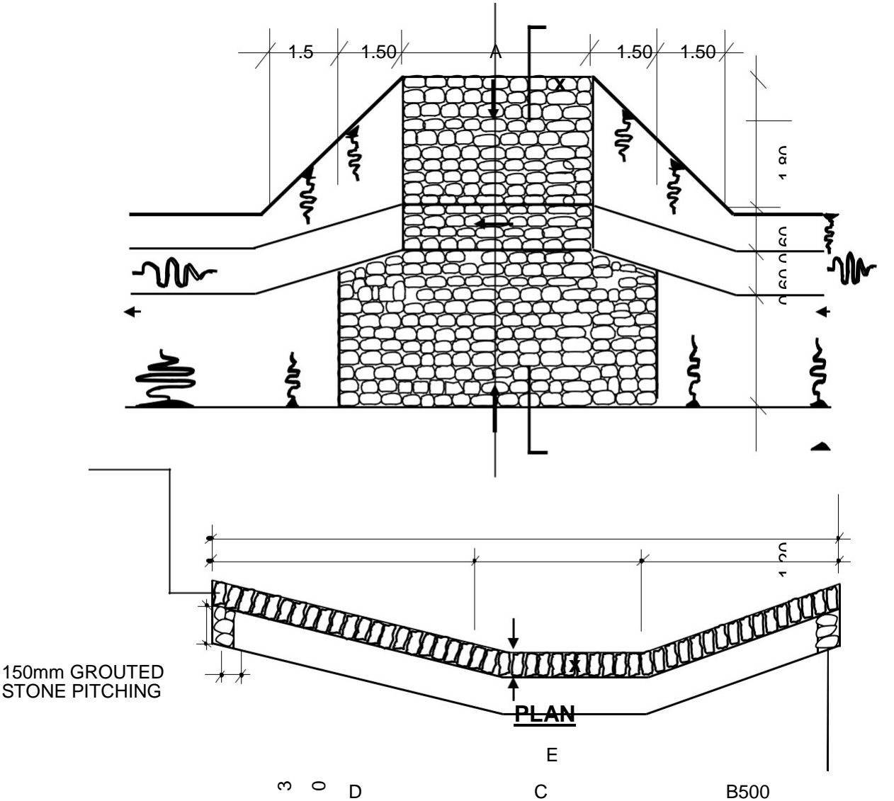
FIGURE C.15 ACCESS DRIFT
