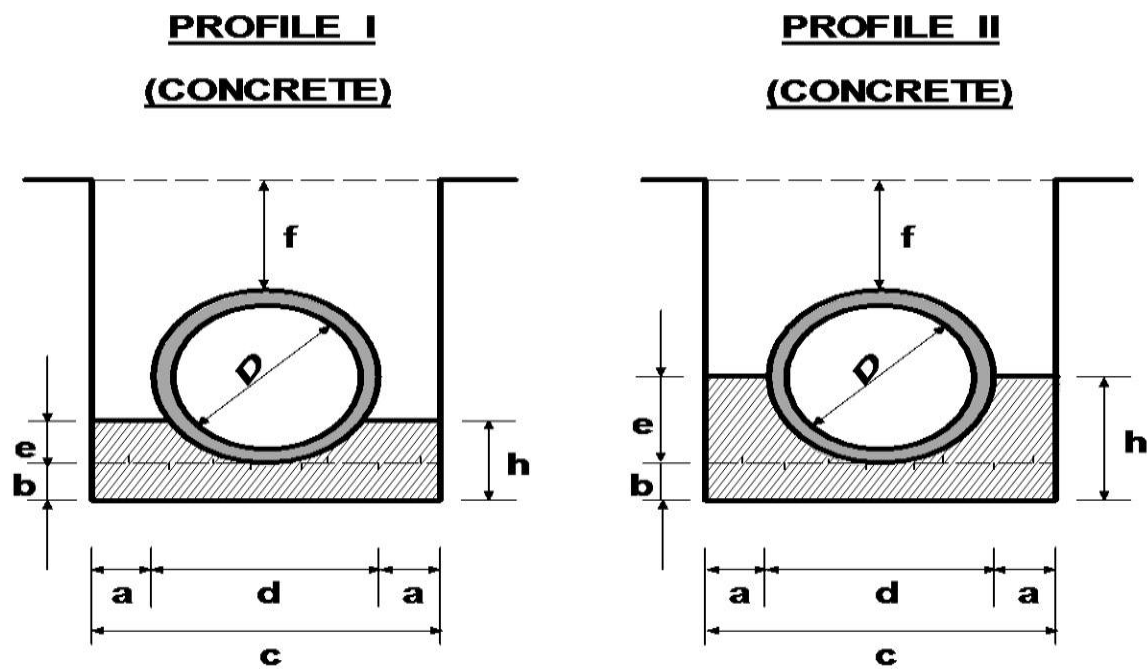
FIGURE C.13- BEDDING AND HAUNCH
