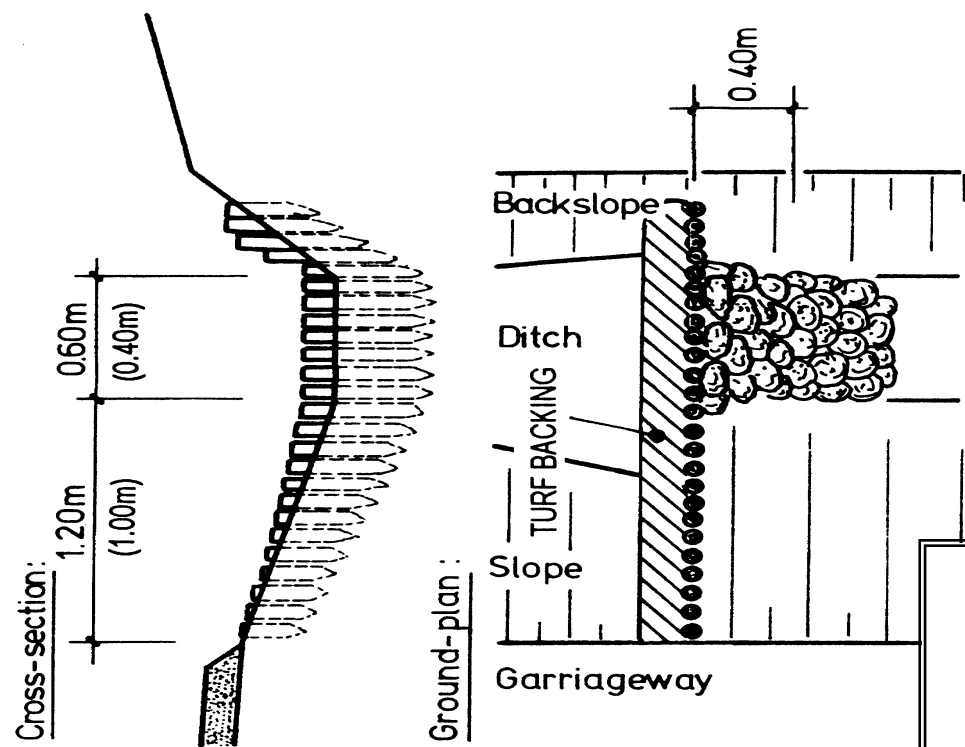
FIGURE C.5 - DIMENSIONS OF SCOUR CHECKS FOR STANDARD DRAIN
