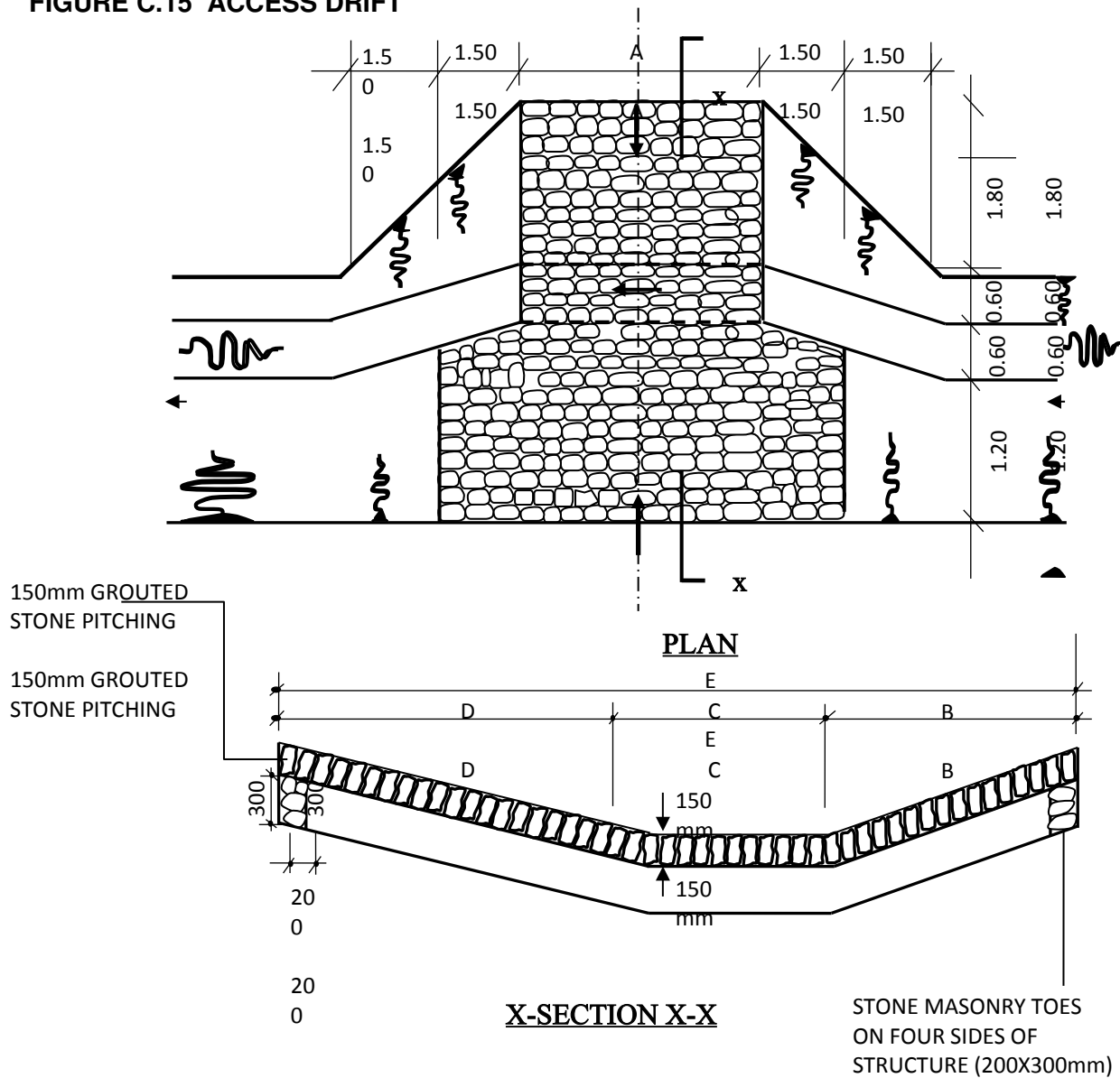
FIGURE C.15 ACCESS DRIFT
