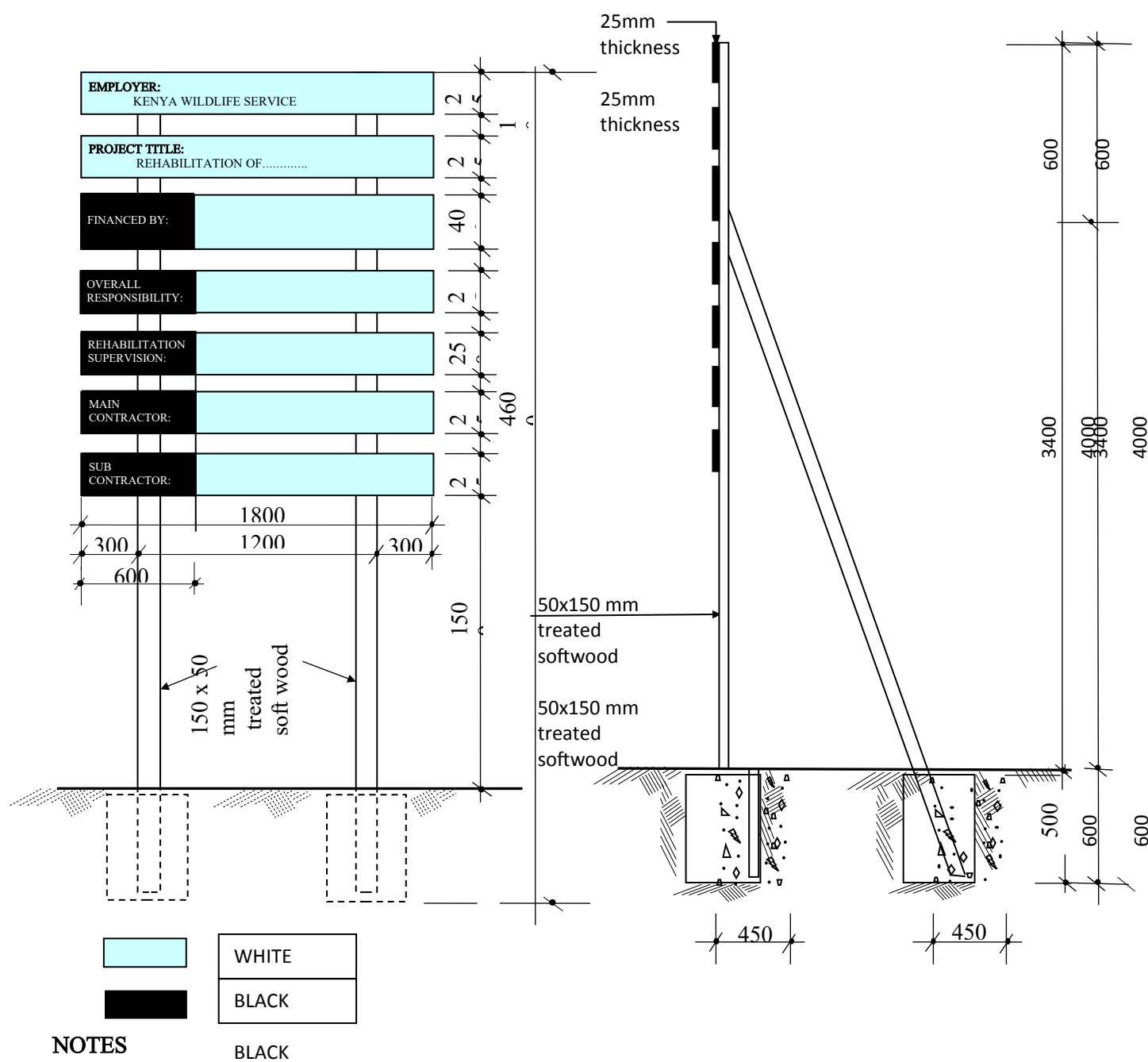
FIGURE C.17 - PUBLICITY SIGNBOARD
