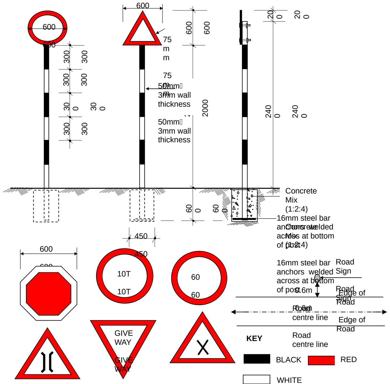
FIGURE C.16 - TRAFFIC SIGNS
