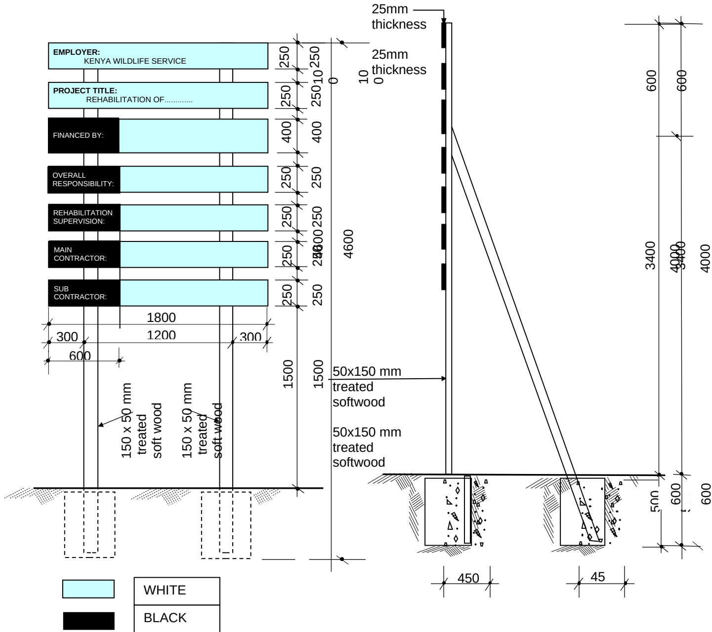
FIGURE C.17 - PUBLICITY SIGNBOARD
