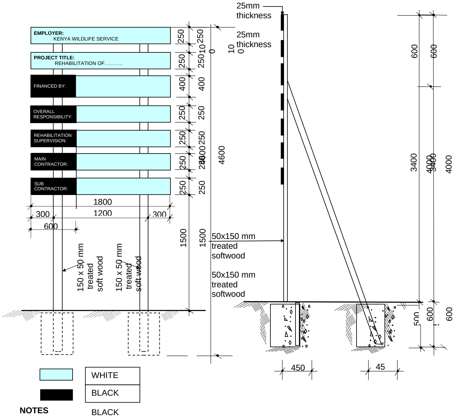
FIGURE C.17 - PUBLICITY SIGNBOARD
