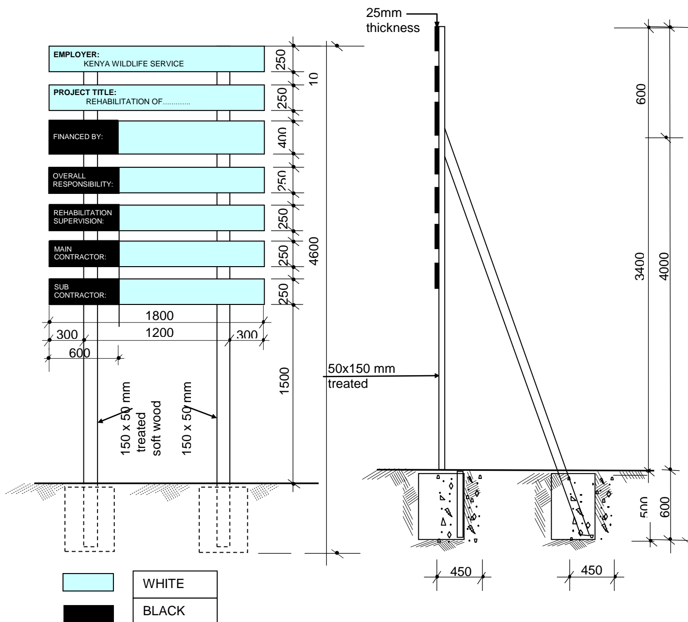
FIGURE C.17 - PUBLICITY SIGNBOARD
