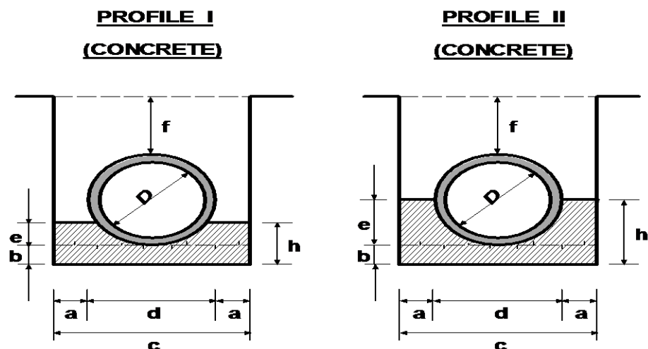
FIGURE C.13- BEDDING AND HAUNCH PROFILES TYPES I & II
