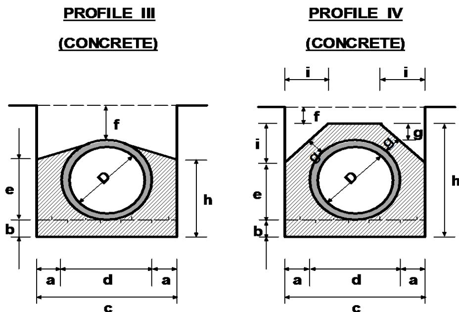
FIGURE C.14 - BEDDING AND HAUNCH PROFILES TYPES III & IV
