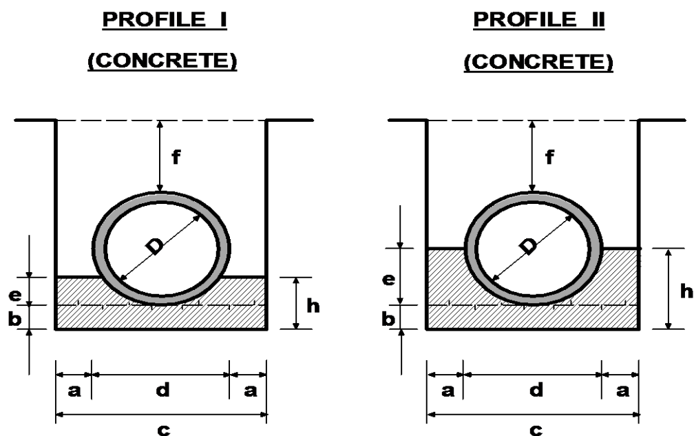
FIGURE C.13- BEDDING AND HAUNCH PROFILES TYPES I & II
