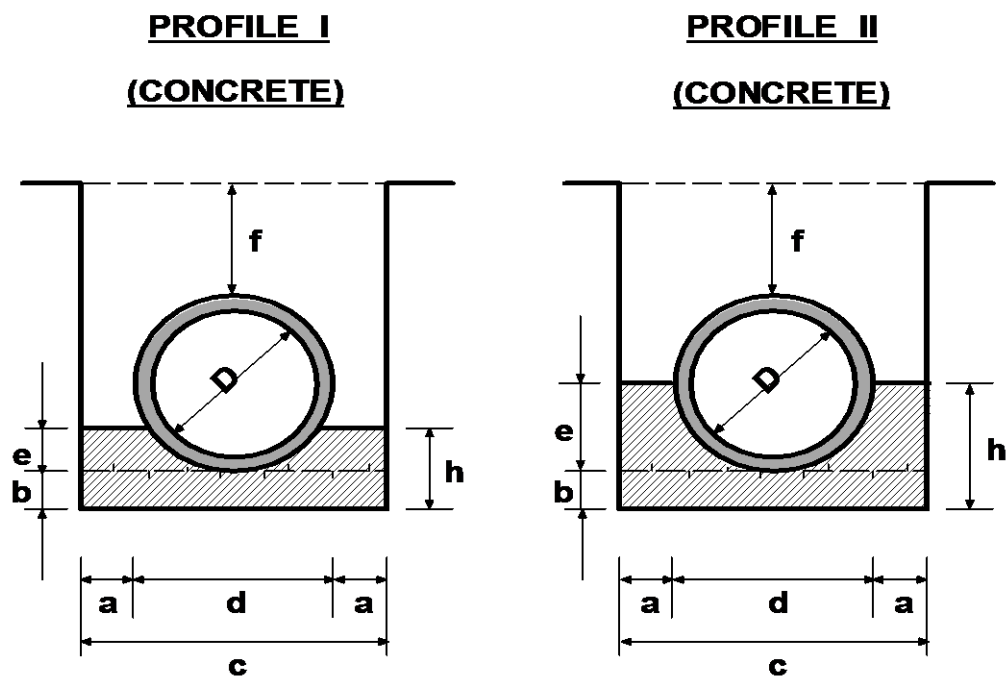
FIGURE C.13- BEDDING AND HAUNCH PROFILES TYPES I & II
