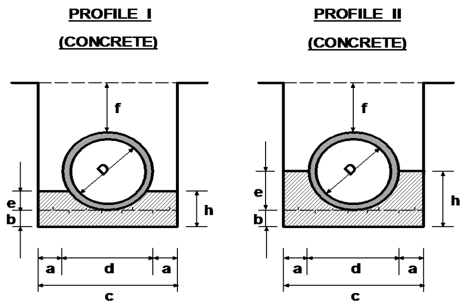
FIGURE C.13- BEDDING AND HAUNCH PROFILES TYPES I & II
