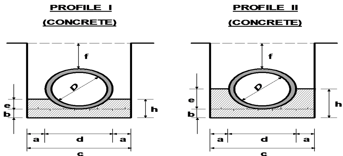
FIGURE C.13- BEDDING AND HAUNCH PROFILES TYPES I & II
