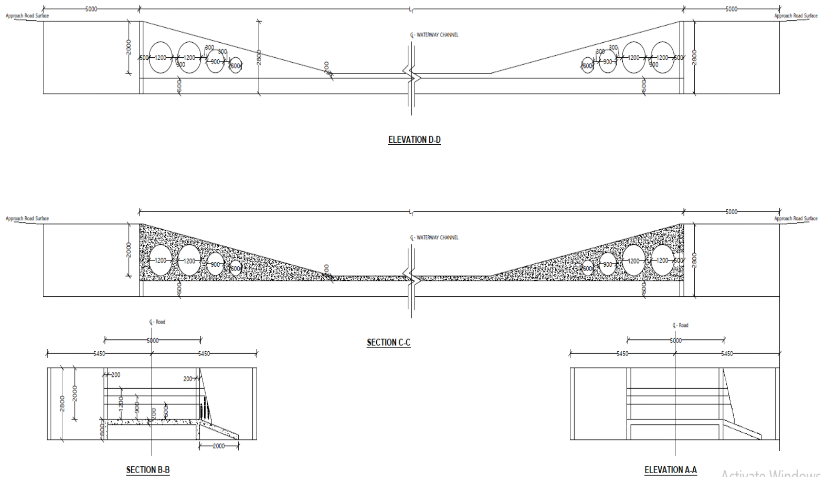
Figure 2-Typical Kitani Drift Details
