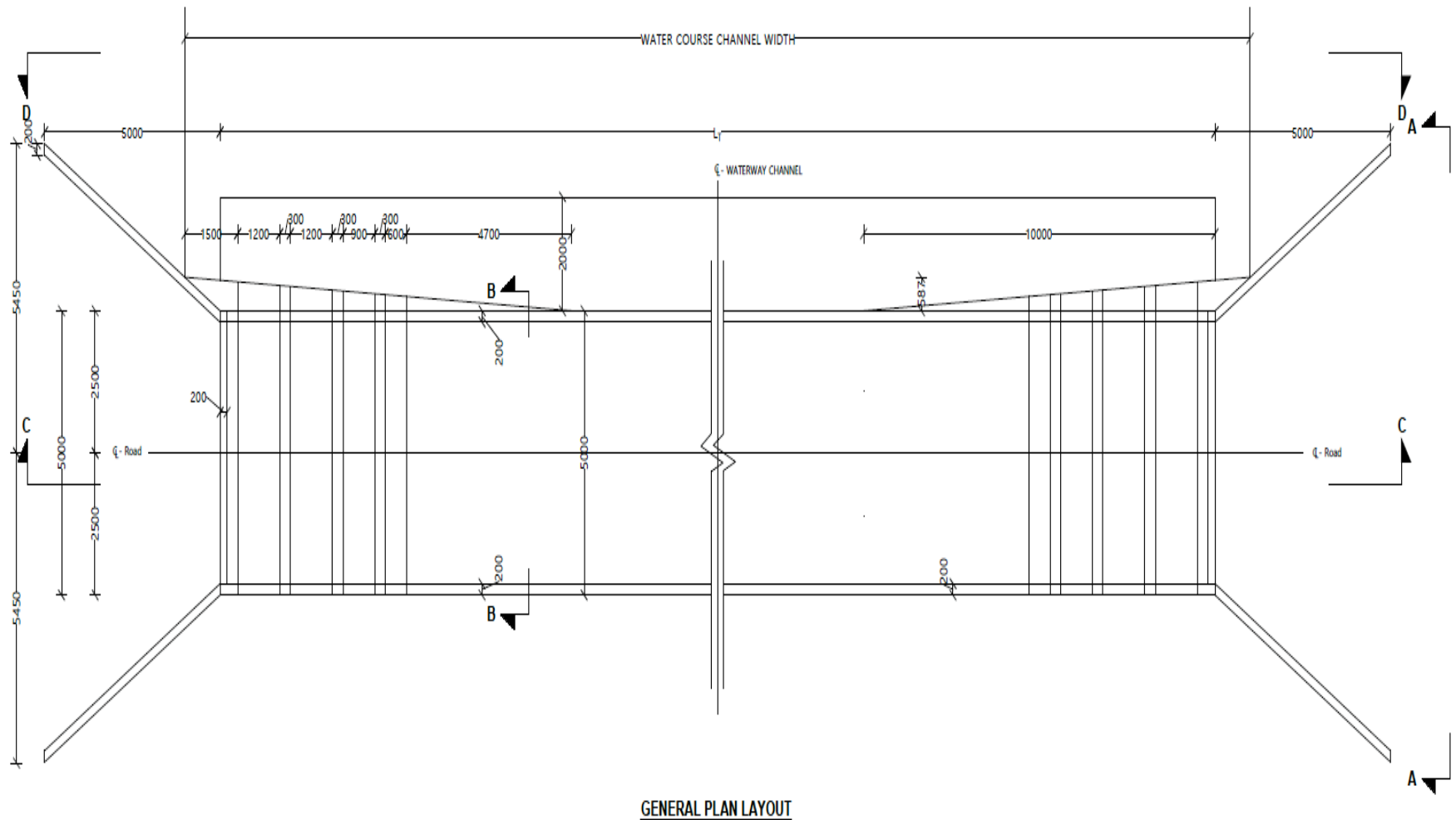
Figure 1-Typical Kitani drift Plan Layout
