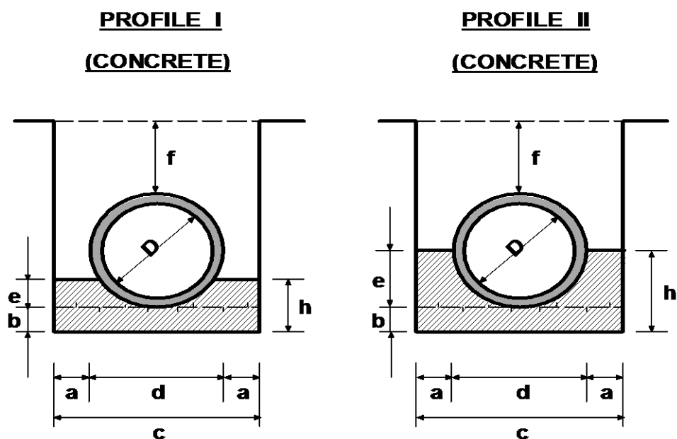
FIGURE C.13- BEDDING AND HAUNCH PROFILES TYPES I & II
