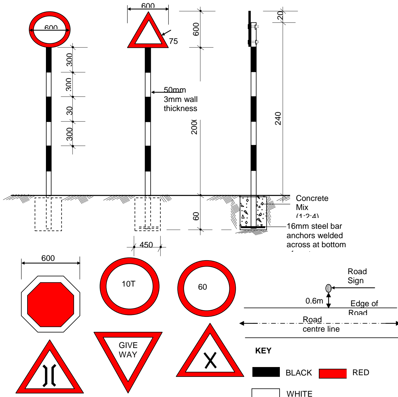
FIGURE C.16 - TRAFFIC SIGNS
