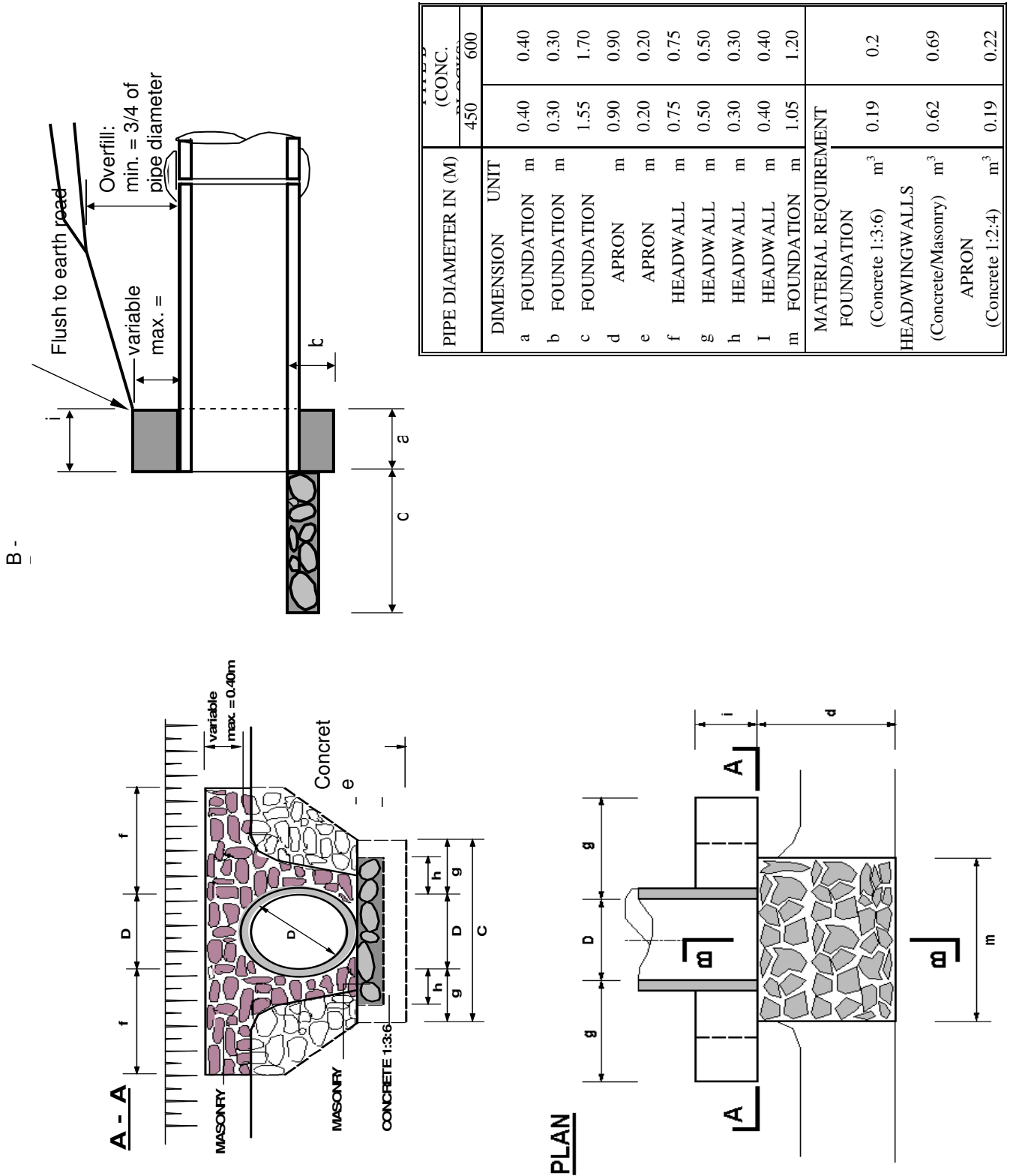
FIGURE C.11 - HEADWALL TYPE 3B (STONE MASONRY HEADWALLS)
