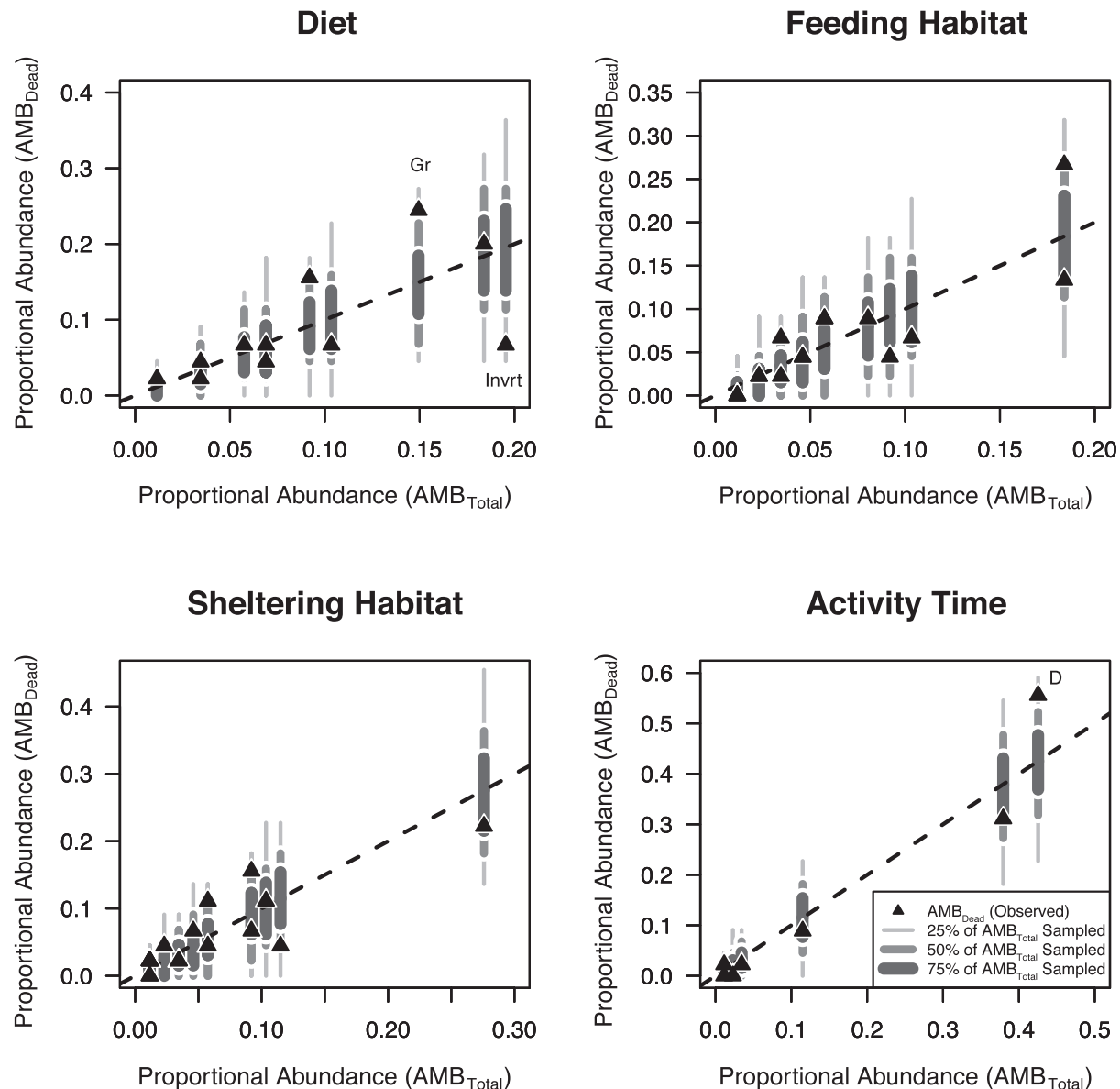
FIGURE 9. Proportional abundances of attributes within each functional ecological trait as recovered by AMB_{Dead} and as simulated through randomized sampling of AMB_{Total} . Error bars are 95% confidence intervals based on Monte Carlo simulations for sampling AMB_{Total} at increasing levels of community completeness (i.e., sampling 25%, 50%, and 75% of all available species). Dashed line shows one-to-one correspondence, representing ideal agreement between AMB_{Total} and AMB_{Dead} . Based on a simulated sampling intensity equal to AMB_{Dead} 's species richness ( S = 45 , 52% of AMB_{Total} richness sampled, Supplementary Table S7), AMB_{Dead} records the proportional abundances of nearly all function attributes within null expectations. Only three functional attributes fall outside expectations: diurnality (D), invertivory (Invrt), and grazing (Gr). These misrepresentations are consistent with AMB_{Dead} 's undersampling of invertebrate-consuming predators (which have complex Activity Times; Fig. 7, Supplementary Fig. S4) and oversampling of large diurnal grazers.
