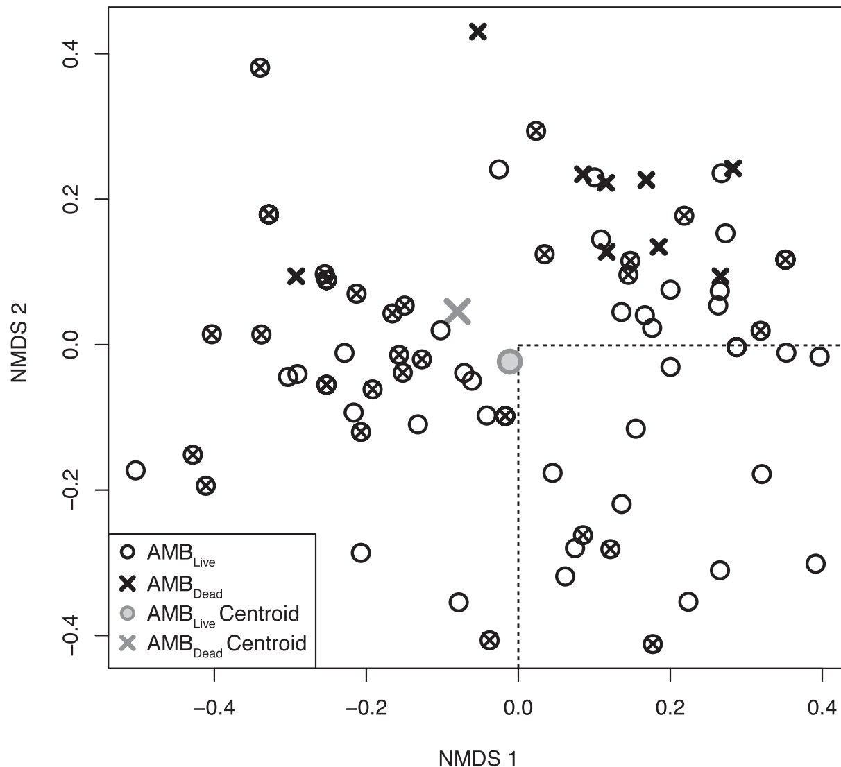
FIGURE 7. Nonmetric multidimensional scaling of four ecological traits for the total Amboseli mammal community ( AMB_{Total} ; Stress = 0.125). Species recorded by AMB_{Death} are small X's. Species documented in AMB_{Live} are open circles. Though not demarcated, the global ( AMB_{Total} ) centroid is located at [0, 0]. A gap in coverage by AMB_{Death} in the lower-right quadrant (dashed box) corresponds to ecospace constructed by species that (1) consume other animals (invertebrates, meat, bone), (2) shelter in underground cavities, and (3) are active during many periods of the day (Supplementary Fig. S2).
